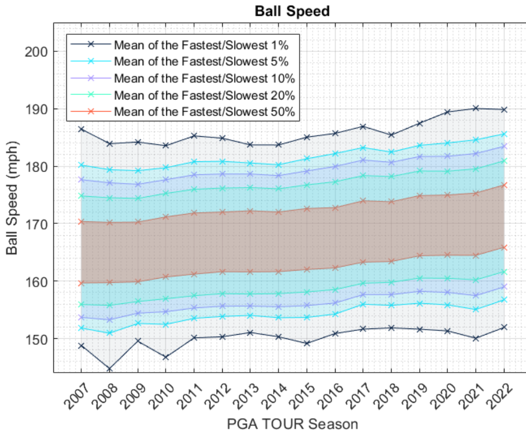
Figure 14. The mean of the fastest and slowest 1%, 5%, 10%, 20% and 50% of measured ball speeds by season on the PGA TOUR.
