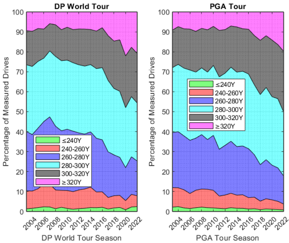
Figure 10. The distribution of drives on “measured” driving holes on the DP World and PGA tours 2003-2022.
